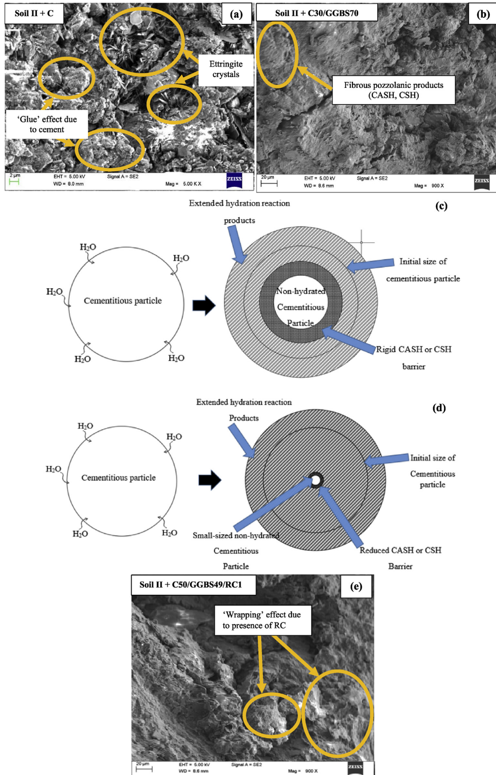
Fig. 4. Mechanism of cement and by-product modified soil: (a) Needle-like ettringite crystals due to cement in stabilised soil; (b) Formed pozzolanic products caused by cement and GGBS addition; (c) Mechanism of stabilisation without inclusion of RC; (d) Mechanism of stabilisation with inclusion of RC; and (e) Transformed stabilised product showing wrapping effect due to RC.
