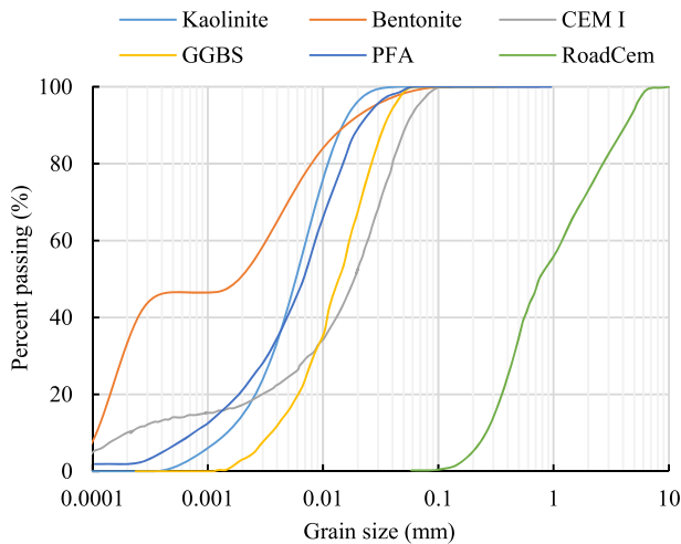
Fig. 1. Analysis of material grain size.
